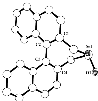
Fig. 1. An ORTEP drawing of 1a . Selected bond lengths, torsion angle ( \text{\AA} , deg): Se1–O1 = 1.642 (9); C1–C2–C3–C4 = -68.0 (2).
